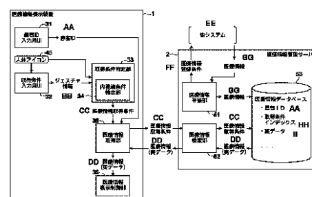
FIG. 4: 1 Medical treatment information display device 2 Medical treatment information management server 31 User interface for patient ID input 32 User interface for acquisition condition input 33 Acquisition condition specification unit 34 Endoscope condition specification unit 35 Medical treatment information acquisition unit 36 Medical treatment information display controller 45 Body icon 61 Medical treatment information registration unit 62 Medical treatment information search unit 53 Medical treatment information database AA Patient ID BB Confirmation information CC Medical treatment information acquisition condition DD Medical treatment information (actual data) EE Other system FF Medical treatment information registration condition GG Medical treatment information HH Acquisition condition index ■ Actual data
